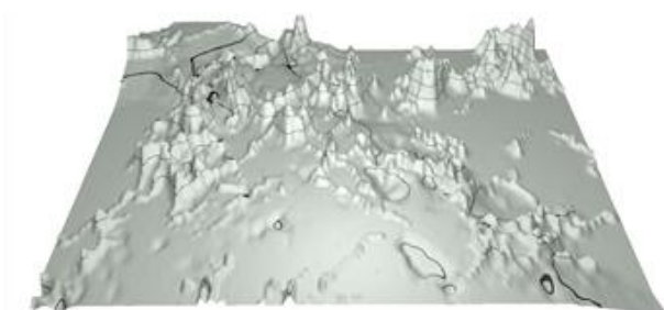
图 7-49. ContourLineStyle = FastColorZones.
