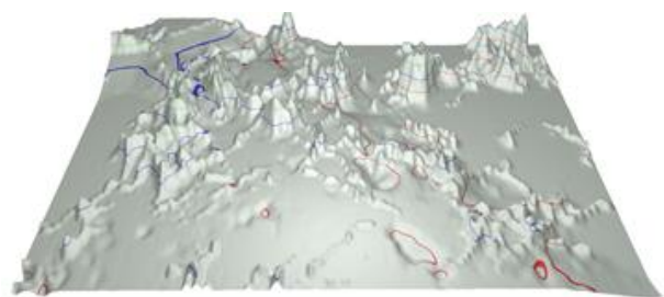
图 7-50. ContourLineStyle = FastPalettedZones.
