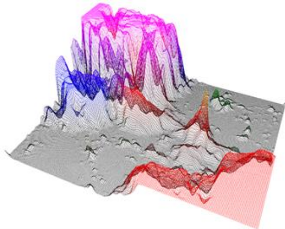
图 7-42. WireframeType = SourcePointColored.
