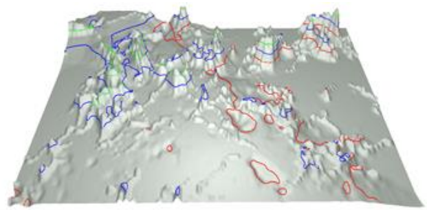
图 7-52. ContourLineType = PalettedLine.
