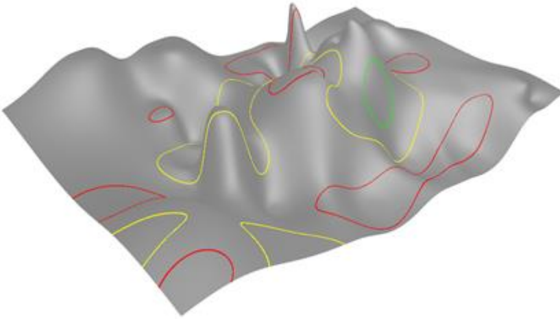
图 7-53. ContourLineType = PalettedLineByValue.
