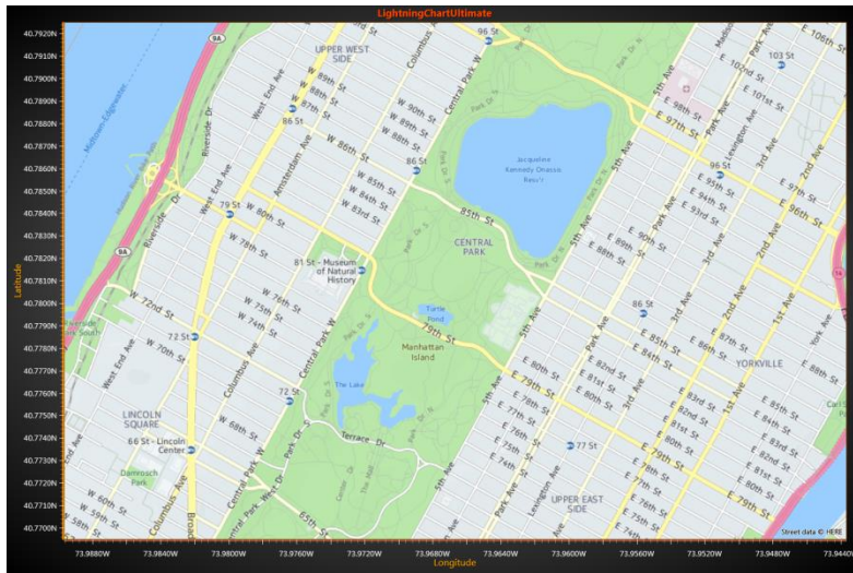
图 6-116. TileLayer.Type = Street .
