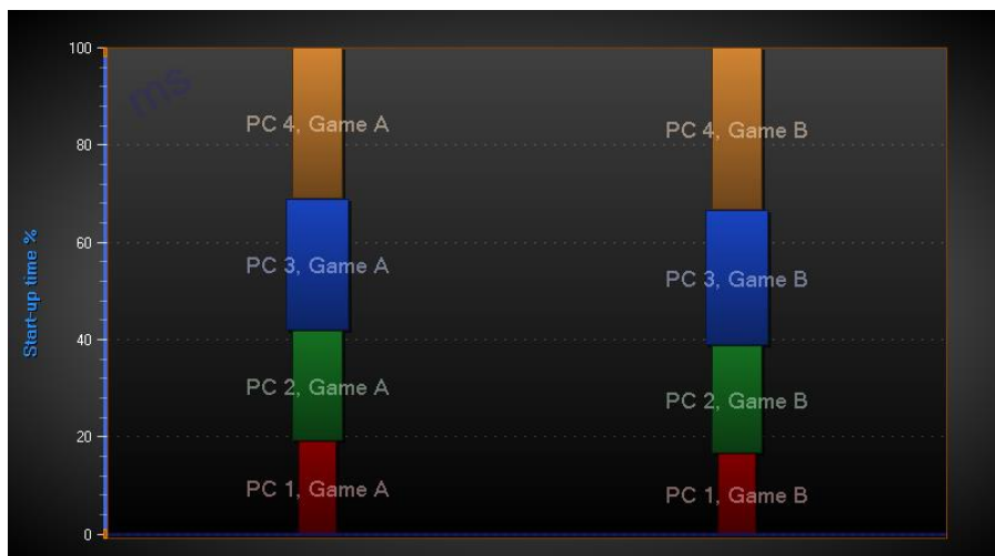
图 6-59. 柱状系列 Grouping = ByIndex , Stacking = StackStretchToSum . StackSum = 100 .
