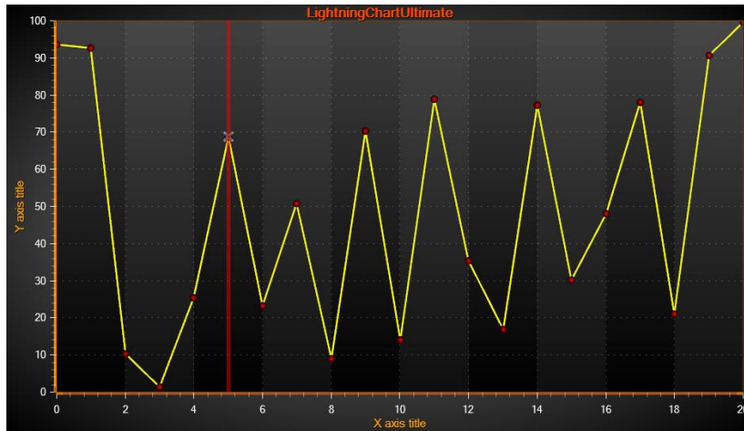
图 6-20. AxisGridStrips = X.
