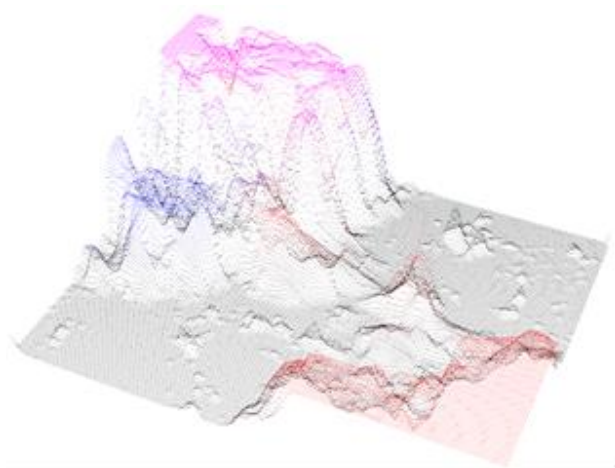
图 7-45. WireframeType = DotsSourcePointColored.
