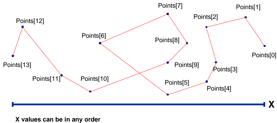
图 6-46. FreeformPointLineSeries 概览
