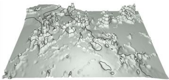
图 7-51. ContourLineType = ColorLine.
