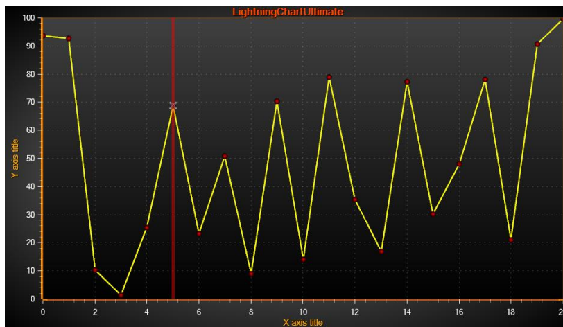
图 6-19. AxisGridStrips = None .
